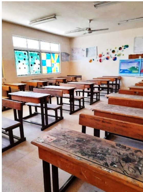
Fig. 3. An interior shot for a base-case classroom. Not all classrooms are equipped with A/Cs; rather, ceiling fans are utilized. Fluorescent tubes are mostly used for lighting classrooms. Also, the single-glazed and aluminum-framed windows are the only type that comprise the building's envelope
