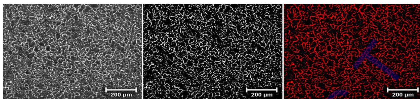
Fig. 18. Optical micrograph of the heat-affected zone preheated at 250 °C: a) grayscale b) threshold c) overlay
