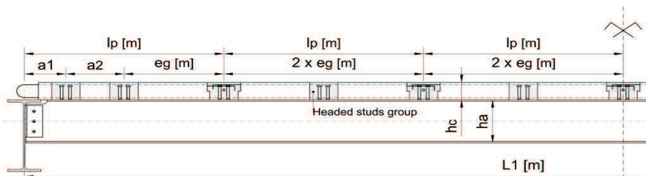
Figure 2: Composite beam with precast RC slab
