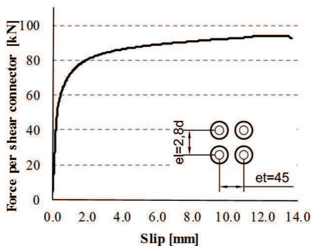
Figure 3: Load – Slip diagram for group of four headed studs d=16\text{mm} h=100\text{ mm}
